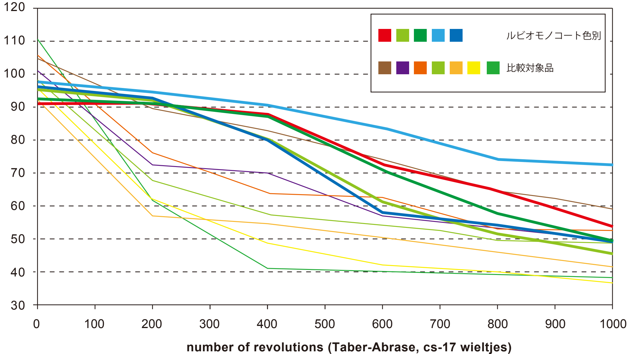
Average contact angle oil finished oak panels
